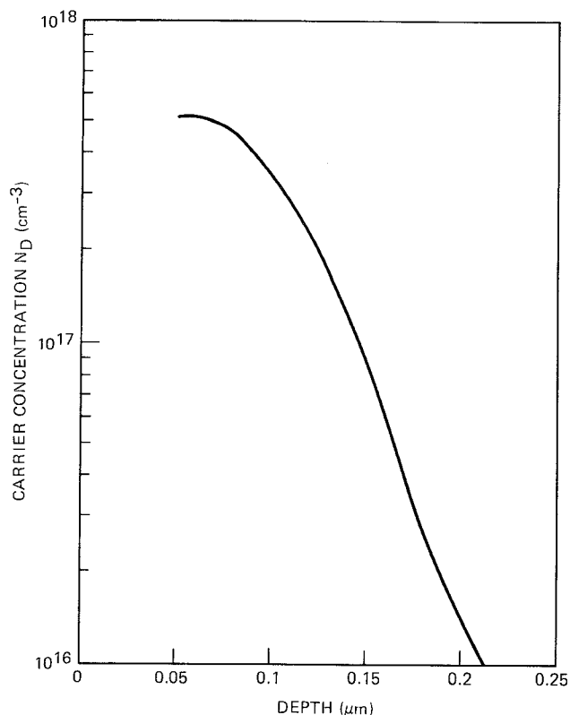
Figure 2. The measured carrier concentration profile from a 70 Kev and 7 \times 10^{12} \text{cm}^{-2} Si + direct ion implantation into a GaAs LEC semi-insulating substrate.
